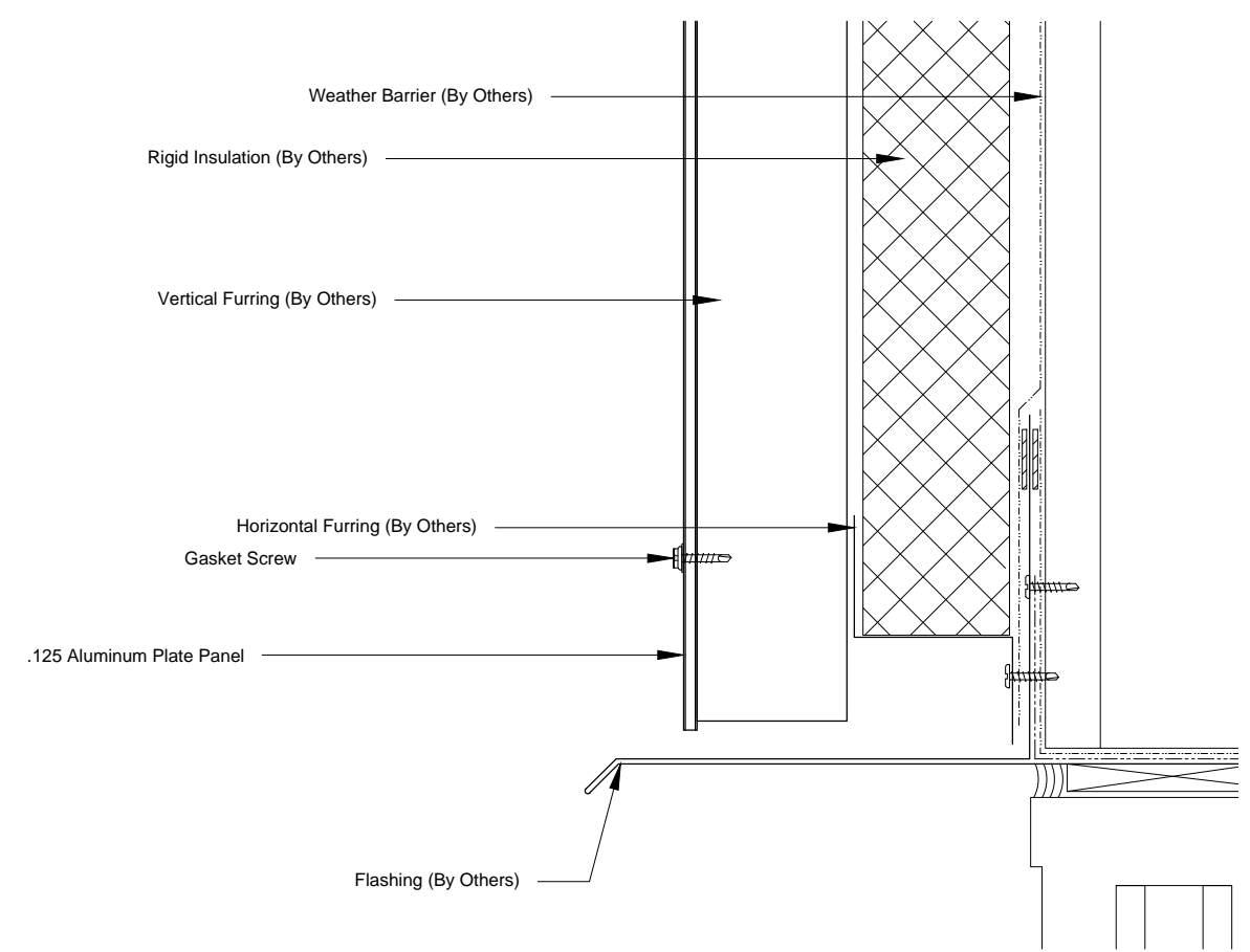
2 Typical Head Detail
