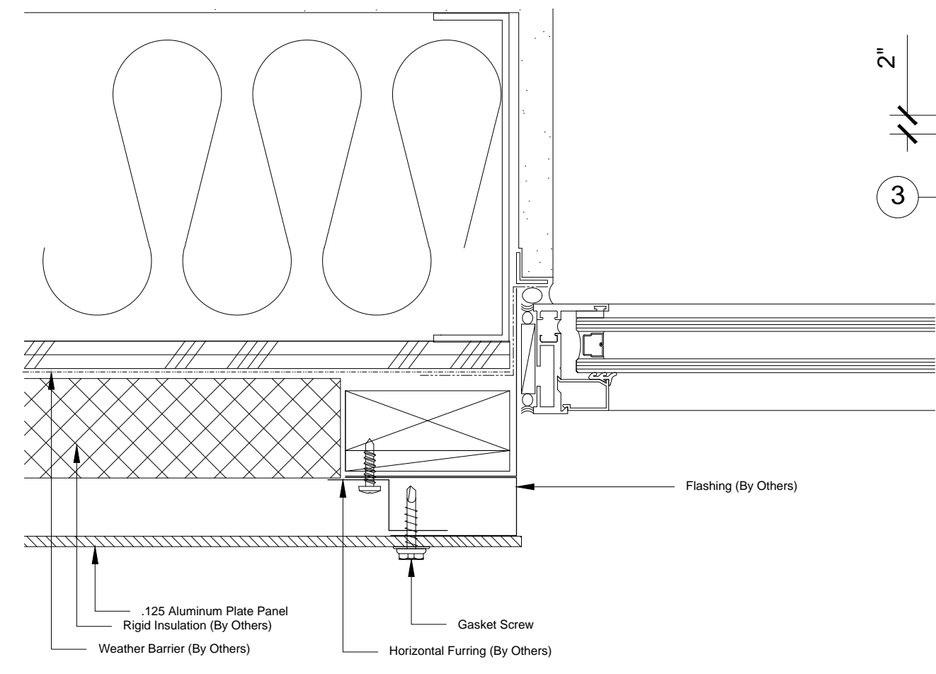
3 Typical Jamb Detail
