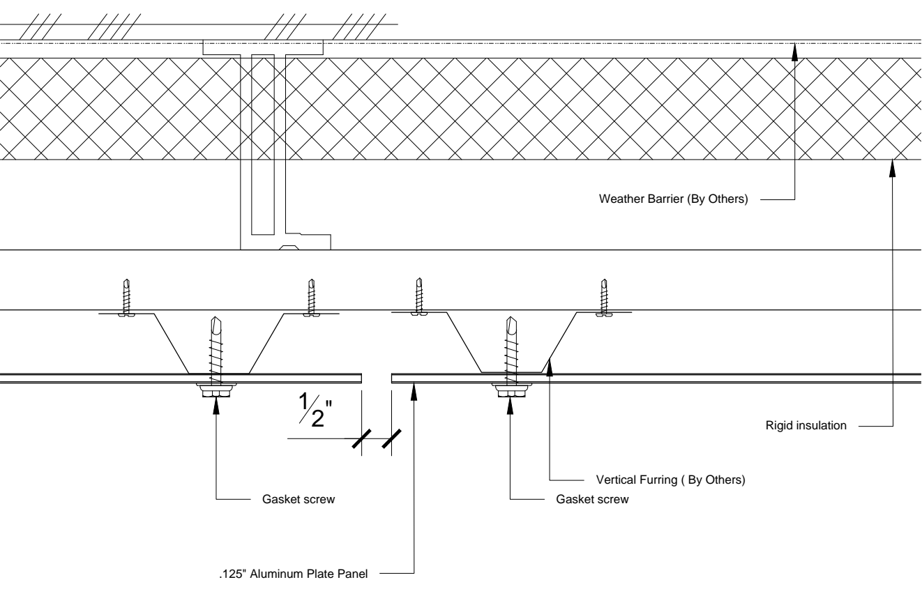
1 Typical Vertical Reveal
